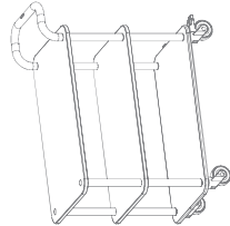
SERVICE CART WITH LEATHER HANDLE L41" W21" H36.5" L104cm W53cm H93cm
