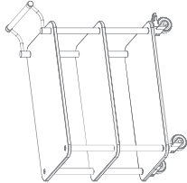
SERVICE CART WITH STAINLESS STEEL HANDLE L41" W21" H36.5" L104cm W53cm H93cm
